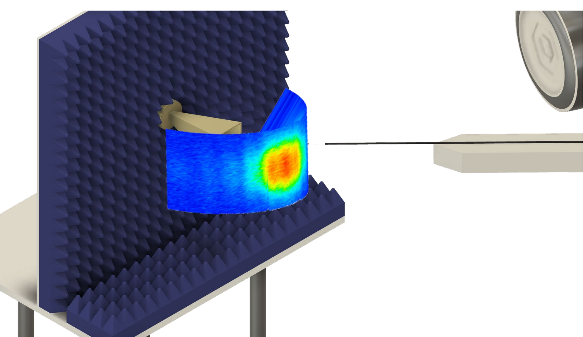
Cylindrical Scanning
